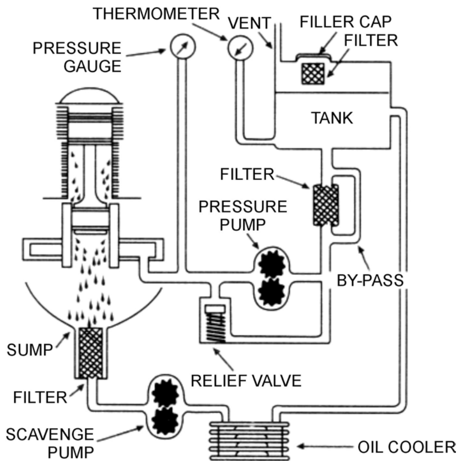
Figure 12C-3 Engine Lubrication
